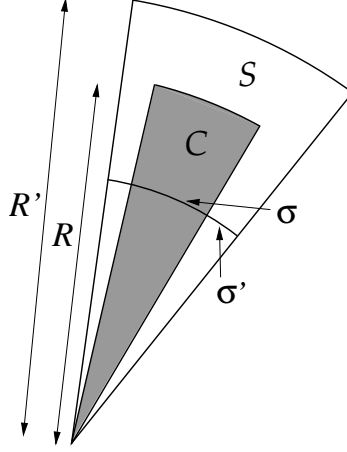
FIGURE 2. Construction of \mathcal{S}, \mathcal{C}
