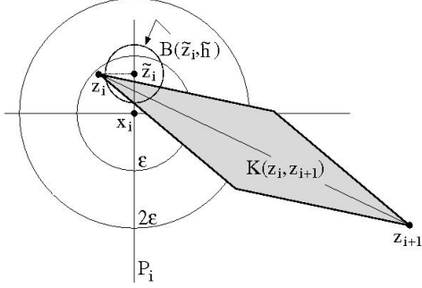
Figure 1. The intersection of the doubly conical region K(z_i, z_{i+1}) with the plane P_i is contained in the ball B(\tilde{z}_i, \tilde{h}) \subset B(x_i, 2\varepsilon) , replacing first [y_j, x_j] and [x_j, x_{j+1}] by [y_j, x_{j+1}] , and next trading [y_j, x_{j+1}] for the union of [y_j, y_{j+1}] and [y_{j+1}, x_{j+1}] . Finally, for j = N we perform two \Delta^{-1} -moves: first replace [y_N, x_N] and [x_N, x_1] by [y_N, x_1] , and then replace [y_N, x_1] and [x_1, y_1] (which has been added at the very beginning of the construction) by [y_N, y_1] . This concludes the whole proof. \square
