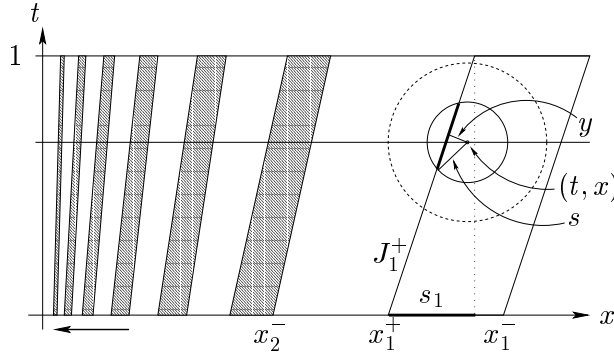
FIGURE 1. Local means (\partial_x u) \star \varphi_s .
