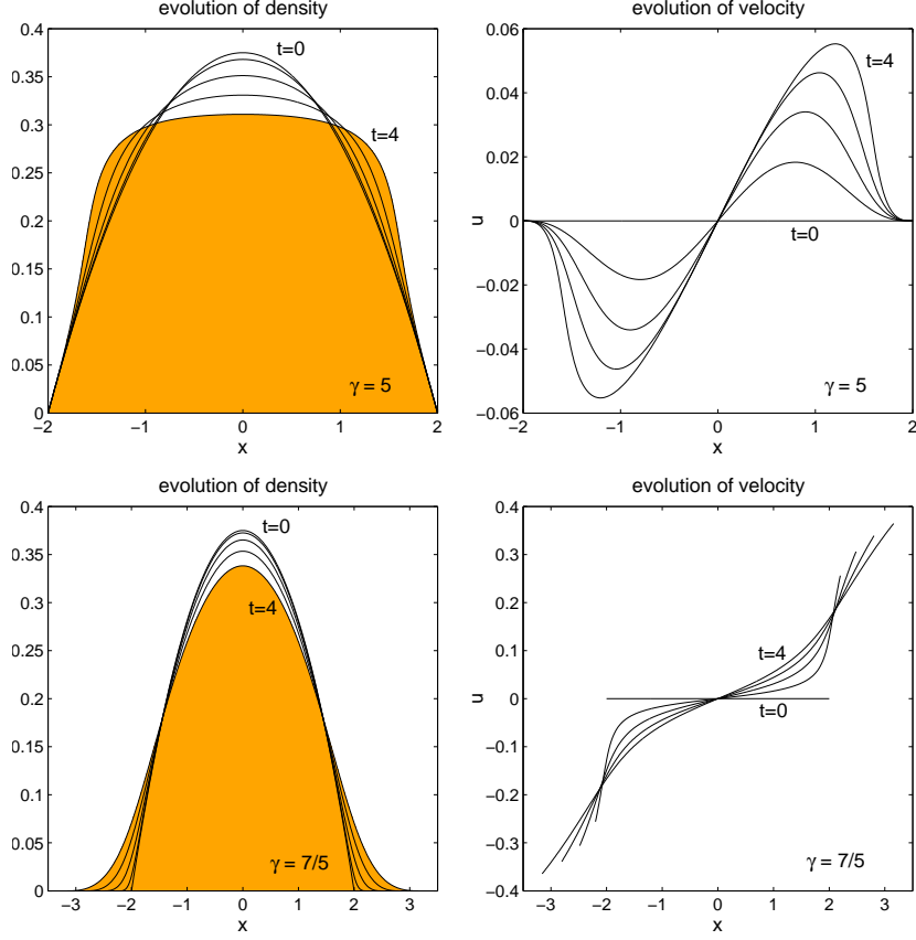
FIGURE 3. Solution of isentropic Euler equations with a parabolic initial distribution of mass, starting from rest. ( N = 800 , VPS2)
