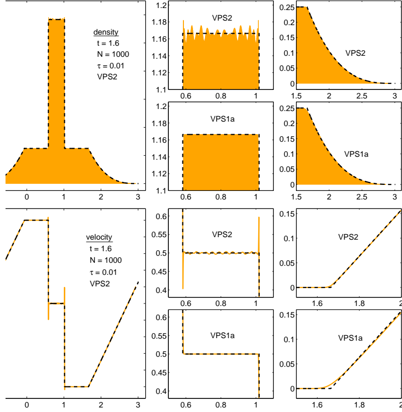
FIGURE 5. Comparison of the VPS2 and VPS1a results with the exact solution of the Riemann problems (dashed lines).
