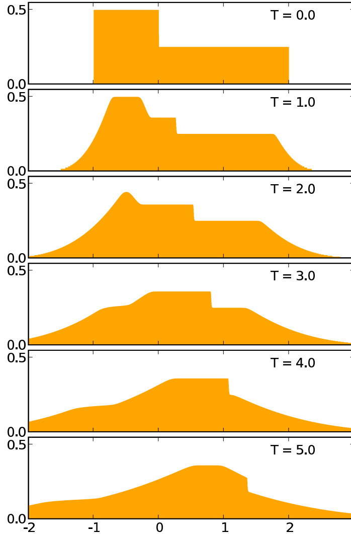
FIGURE 7. Isentropic Euler equations with \gamma = 5/3 .
